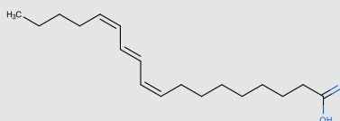
Punicic acid
