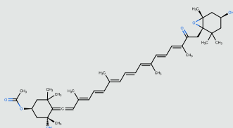
Fucoxanthin
